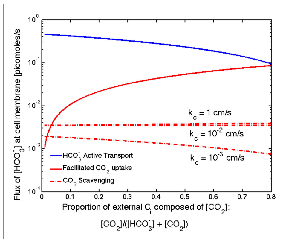
Figure 5. Size of the \text{HCO}_3^- flux in one cell from varying sources, as the proportion of \text{CO}_2 to \text{HCO}_3^- outside the cell changes. We show results for three carboxysome permeabilities, k_c , and only the scavenging is effected.
