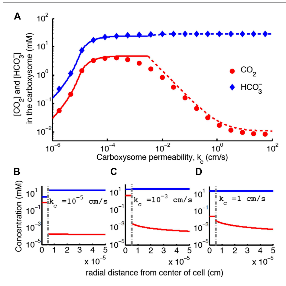
Figure 4. Concentration of CO 2 in the carboxysome with varying carboxysome permeability (A). Numerical solution (diamonds and circles) and analytic solutions (carbonic anhydrase unsaturated, solid lines, and saturated, dashed lines) correspond well. On all plots CO 2 (red circle) < HCO 3 - (blue diamond). Concentration in the cell along the radius, r , with carboxysome permeability k_c = 10^{-5} \frac{cm}{s} (B), k_c = 10^{-3} \frac{cm}{s} (C), k_c = 1 \frac{cm}{s} (D). Grey dotted lines in (B), (C), (D) indicate location of the carboxysome shell boundary. The transition from low CO 2 at high permeability (D) to maximum CO 2 concentration at optimal permeability (C) occurs at k_c^* = \frac{D}{R_c} = 2 \frac{cm}{s} . At low carboxysome permeability (B) HCO 3 - diffusion into the carboxysome is slower than consumption. For all subplots \alpha = 0 \frac{cm}{s} and j_c = 0.6 \frac{cm}{s} . Qualitative results remain the same with varying j_c , increasing \alpha will increase the gradient of CO 2 across the cell as CO 2 is converted to HCO 3 - at the cell membrane.
