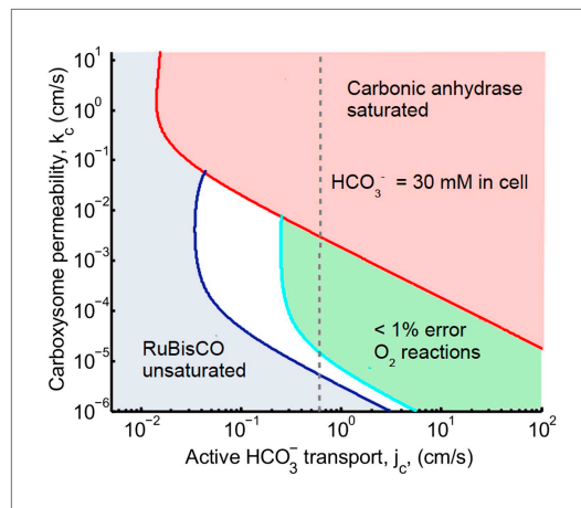
Figure 2. Phase space for \text{HCO}_3^- transport, j_c and carboxysome permeability k_c . Plotted are the parameter values at which the \text{CO}_2 concentration reaches some critical value. The left most line (dark blue) indicates for what values of j_c and k_c the \text{CO}_2 concentration in the carboxysome would half-saturate RuBisCO ( K_m ). The middle line (light blue) indicates the parameter values which would result in a \text{CO}_2 concentration where 99% of all RuBisCO reactions are carboxylation reactions and only 1% are oxygenation reactions when \text{O}_2 concentration is 260 \mu\text{M} . The right most (red) line indicates the parameter values which result in carbonic anhydrase saturating. Here \alpha = 0 , so there is no \text{CO}_2 scavenging or facilitated uptake. The dotted line (grey) shows the k_c and j_c values, where the \text{HCO}_3^- concentration in the cytosol is 30 \text{ mM} . The \text{HCO}_3^- concentration in the cytosol does not vary appreciably with k_c in this parameter regime, and reaches 30 \text{ mM} at j_c \approx 0.6 \frac{\text{cm}}{\text{s}} . All other parameters, such as reaction rates are held fixed and the value can be found in the Table 1 and Table 2 .
