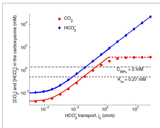
Figure 3. Numerical solution (diamonds and circles) and analytic solutions (carbonic anhydrase unsaturated, solid lines, and saturated, dashed lines) correspond well. \text{HCO}_3^- transport is varied, and all other system parameters are held constant. The \text{CO}_2 concentration above which RuBisCO is saturated is K_m (grey dashed line). The \text{CO}_2 concentration where the oxygen reaction error rate will be 1% is C_{99\%} (grey dash-dotted line). The transition between carbonic anhydrase being unsaturated and saturated happens where the two analytic solutions meet (where the dashed and solid red lines meet). Below a critical value of transport, j_c \approx 10^{-3} \frac{\text{cm}}{\text{s}} the level of transport is lower than the \text{HCO}_3^- leaking through the cell membrane. A value of k_c = 10^{-3} \frac{\text{cm}}{\text{s}} for the carboxysome permeability was used for these calculations.
