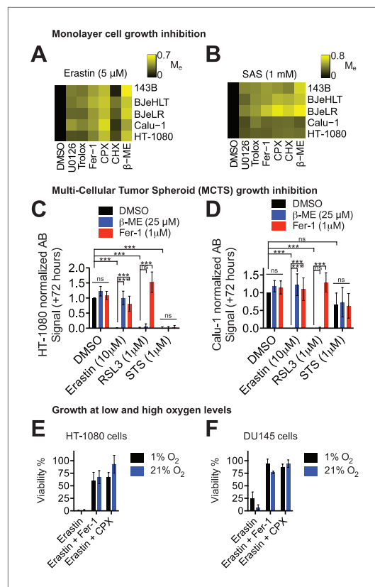
Figure 1. Cell death is triggered by erastin and related compounds in different cell lines under a variety of physiological conditions. (A and B) Modulatory effect ( M_e ) profiles of erastin- and SAS-induced death in five different cell lines (143B, BJeHLT, BJeLR, Calu-1, and HT-1080) in response to six different cell death inhibitors (U0126, Trolox, Fer-1, CPX, CHX, \beta -ME) or the vehicle DMSO. M_e > 0 indicates rescue from cell death. (C and D) Relative viability of MCTSs formed over 72 hr from HT-1080 (C) or Calu-1 (D) cells in response to erastin, RSL3 or staurosporine (STS) \pm \beta -ME or ferrostatin-1 (Fer-1). Viability was assessed by Alamar blue and represents mean \pm SD from three independent biological replicate experiments. Data were analyzed by two-way ANOVA with Bonferroni post-tests, * p < 0.05 , ** p < 0.05 , *** p < 0.001 , ns = not significant. (E and F) Viability of HT-1080 (E) and DU145 (F) cells cultured under 1% or 21% O_2 levels in response to erastin (5 \mu M) \pm Fer-1 (1 \mu M) or CPX (5 \mu M). Viability was assessed by Alamar blue and represents mean \pm SD from three independent biological replicate experiments.
