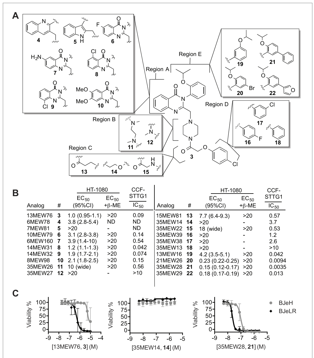
Figure 3. Structure activity relationship (SAR) analysis of erastin. (A) Structures of 20 erastin analogs. (B) Lethal EC 50 for each analog determined in HT-1080 cells in a 10-point, twofold dilution assay, starting at a high concentration of 20 μM, ±β-ME (18 μM). Data represent mean and 95% confidence interval (95% C.I.) from three independent biological replicate experiments. Also reported are IC 50 values for inhibition of glutamate release as determined in CCF-STTG1 cells. These data represent the average of two experiments. All values are in μM. ND: not determined. (C) Dose-response curves for selected erastin analogs ( 3 , 14 and 21 ) in BJeLR and BJeH cells. Data represent mean ± SD from three independent biological replicates.
