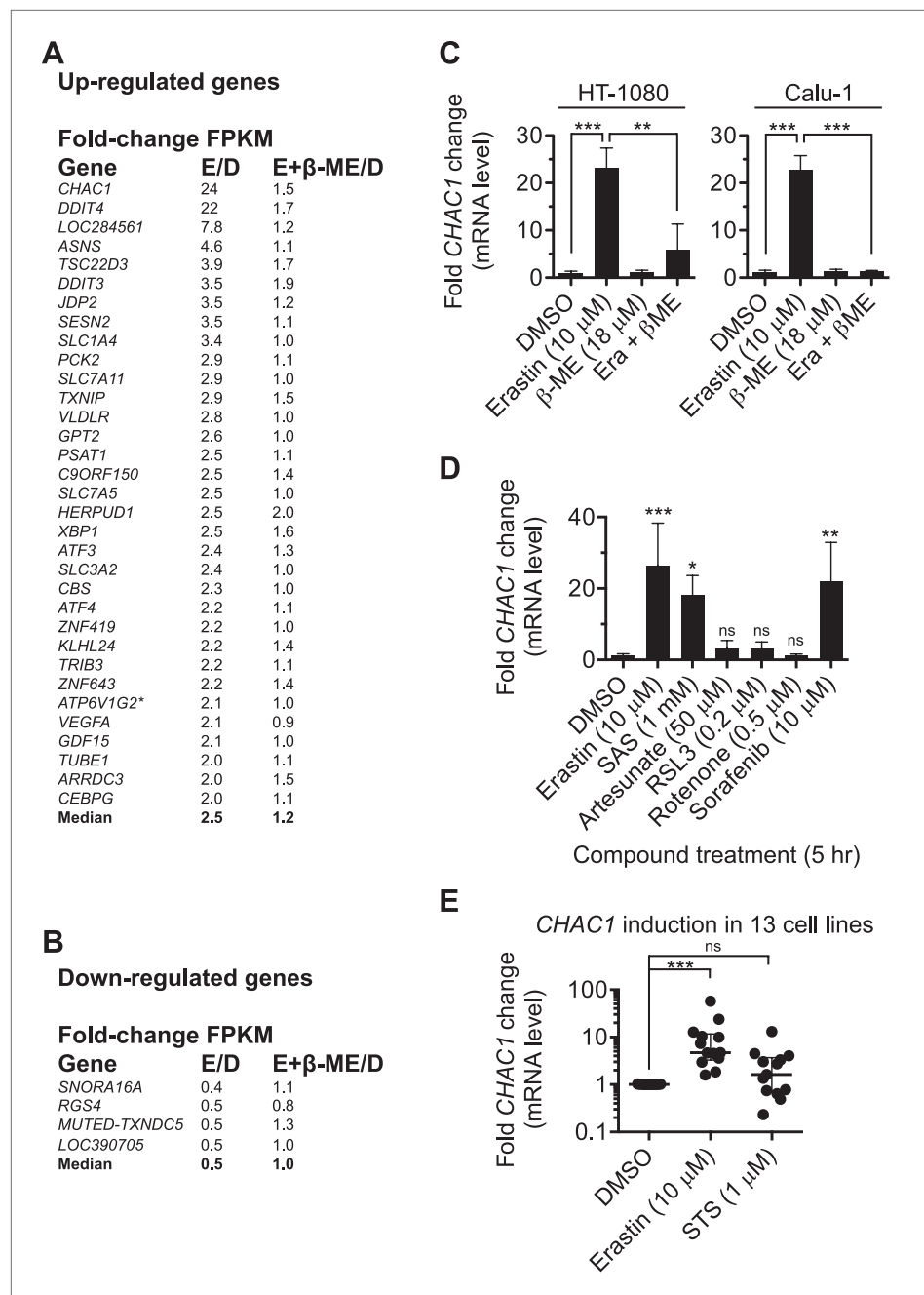
Figure 4. Analysis of erastin effects using RNA-Seq. (A and B) List of genes upregulated (A) and downregulated (B) by erastin treatment, as detected in HT-1080 cells using RNA Seq. The number of fragments per kilobase of exon per megabase of sequence (FPKM) was counted and is expressed as a fold-change ratio between the different conditions. E/D: Erastin/DMSO expression ratio. E+β-ME/D: Erastin+β-ME/DMSO ratio. ATP6V1G2* : ATP6V1G2-DDX39B read-through transcript. Data represent the average of two independent biological replicates for each condition. (C and D) mRNA expression level of CHAC1 determined by RT-qPCR in HT-1080 and Calu-1 cells in response to erastin ±β-ME treatment for 5 hr. Data are from three independent biological replicates and represented as mean ± SD and were analyzed by one-way ANOVA with Bonferroni post-tests, ** p < 0.01 , *** p < 0.001 , ns = not significant. In D significance is indicated relative to the DMSO control. (E) CHAC1 mRNA levels in 13 different erastin-sensitive cell lines treated with erastin or STS (6 hr). Results in E were analyzed using the Kruskal–Wallis test, *** p < 0.001 , ns = not significant.
