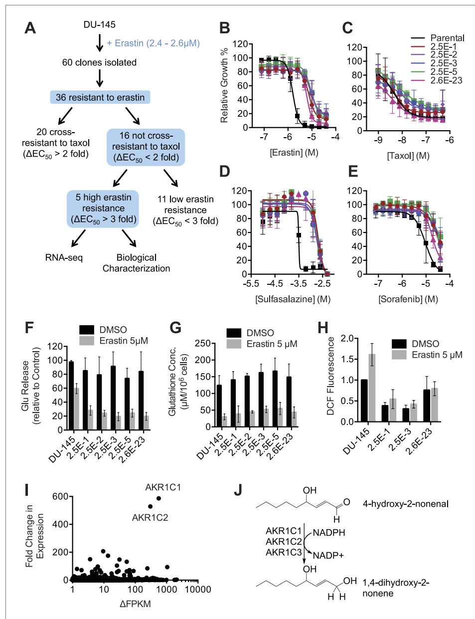
Figure 8. Isolation and analysis of erastin-resistant clones identifies AKR1C genes as mediators of resistance to system x_c^- inhibition. (A) Outline of the isolation of DU-145 erastin-resistant clones. (B–H) Comparison of the parental DU-145 cell line and five erastin-resistant clonal lines to the indicated lethal compounds: (B–E) , response to different lethal compounds, (F) Glutamate release, (G) Glutathione concentration, (H) DCF fluorescence. (I) Summary of RNA Seq analysis of the five erastin-resistant clones vs the parental DU-145 cells. Fold-change in expression (y-axis) and absolute change in FPKM (x-axis) is computed from the average of the five resistant cells lines vs parental. (J) Summary of AKR1C family member activity possibly relevant to ferroptosis. DOI: 10.7554/eLife.02523.014
