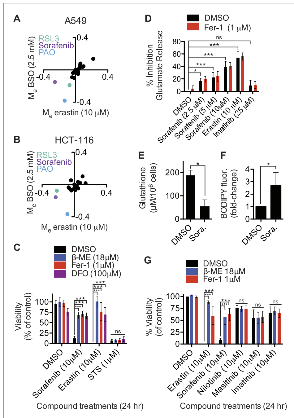
Figure 5. Identification of sorafenib as an inhibitor of system x_c^- . (A and B) Modulatory profiling of (A) A549 and (B) HCT-116 cells in response to either buthionine sulfoximine (BSO) or erastin \pm 20 different lethal compounds (see 'Materials and methods' for the full list). (C) Viability of HT-1080 cells treated for 24 hr with ferroptosis inhibitors ( \beta -ME, Fer-1, DFO) \pm sorafenib, erastin or STS. (D) Quantification of the inhibition of glutamate release by sorafenib, erastin and imatinib \pm Fer-1. (E and F) HT-1080 cells treated with control vehicle (DMSO) or sorafenib (10 \mu M) for 18 hr prior to the assay. (E) Total glutathione levels measured using Ellman's reagent. (F) Lipid ROS levels assayed using C11-BODIPY 581/591. (G) Viability of HT-1080 cells treated for 24 hr with erastin, sorafenib, nilotinib, masitinib or imatinib \pm \beta -ME or Fer-1. Data in C–G represent mean \pm SD from at least three independent biological replicates. Cell viability in C and G was quantified by Alamar blue. Data in C, D and G were analyzed by one- and two-way ANOVA with Bonferroni post-tests; data in E and F were analyzed using Student's ttest, * p <0.05, ** p <0.01, *** p <0.001, ns = not significant relative to the indicated treatments. In (D), none of the comparisons between DMSO and Fer-1 treated samples were significant ( p >0.05).
