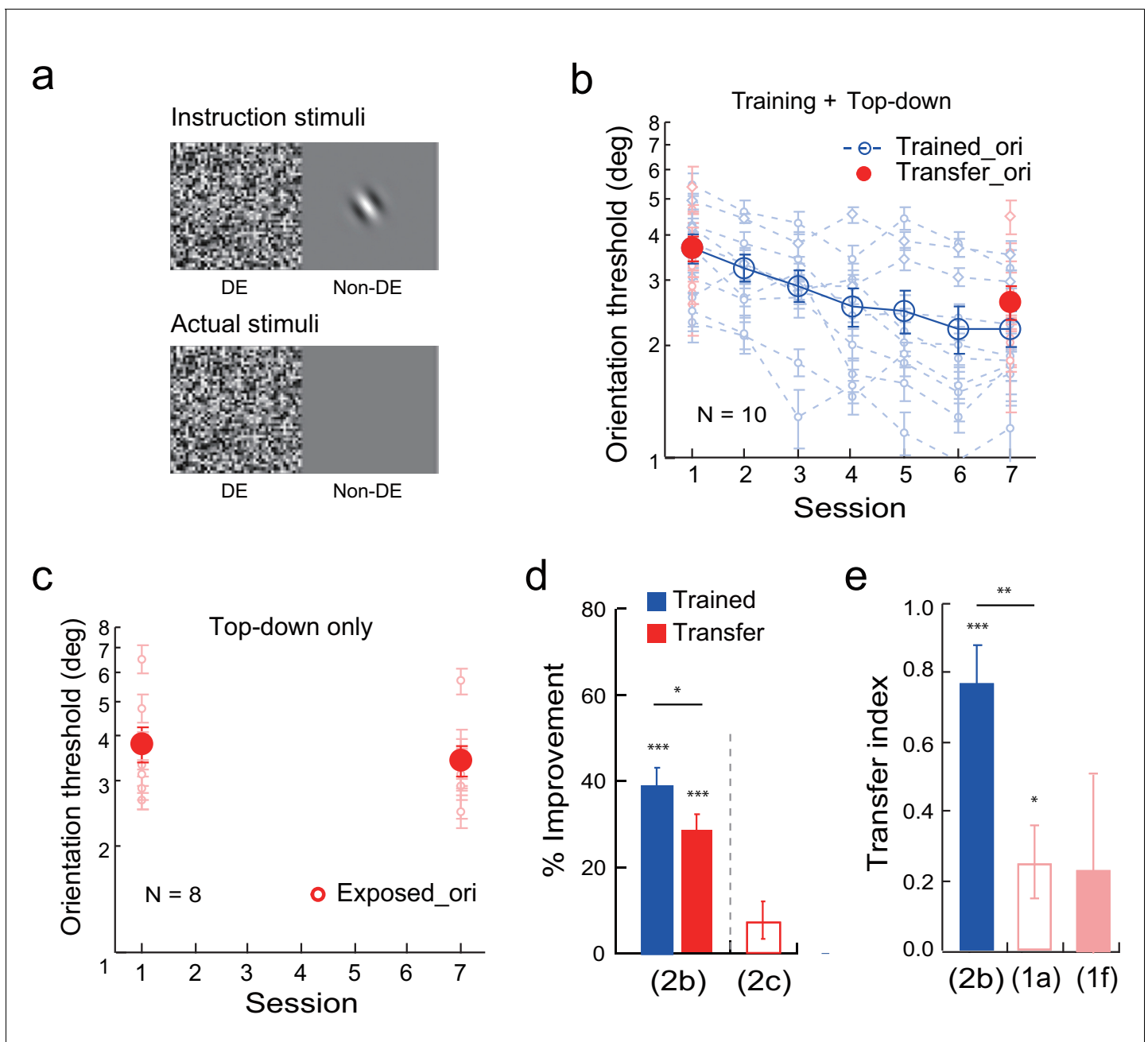
Figure 2. Orientation discrimination learning and the effect of top-down attention to the transfer orientation on learning transfer. (a) CFS configurations for the top-down attention condition. Instruction stimuli: Before the experiment the observers were instructed through a demo that an orthogonal Gabor or an uppercase letter C would be presented to the non-dominant eye, and that they needed to report whether it was a Gabor or a C even if they could not perceive it. Actual stimuli: In actual testing the Gabor/C was replaced by a blank screen. Orientation discrimination training and the top-down attention condition were conducted in different blocks of trials. (b) The mean and individual learning and transfer data with training and top-down attention to the transfer orientation. (c) Control experiment. Same as 2b except that there was no orientation discrimination training. (d) A summary of learning and transfer in the top-down attention and control conditions. (e) A summary of the transfer indices in the current training plus top-down attention condition and the previous baseline (replotted from Figure 1a ) and training plus noise-only (replotted from Figure 1f ) conditions. Error bars indicate \pm 1 standard error of the mean. DE - dominant eye. * p < 0.05 ; ** p < 0.01 ; *** p < 0.001 . See Figure 2—source data 1 for raw data.
