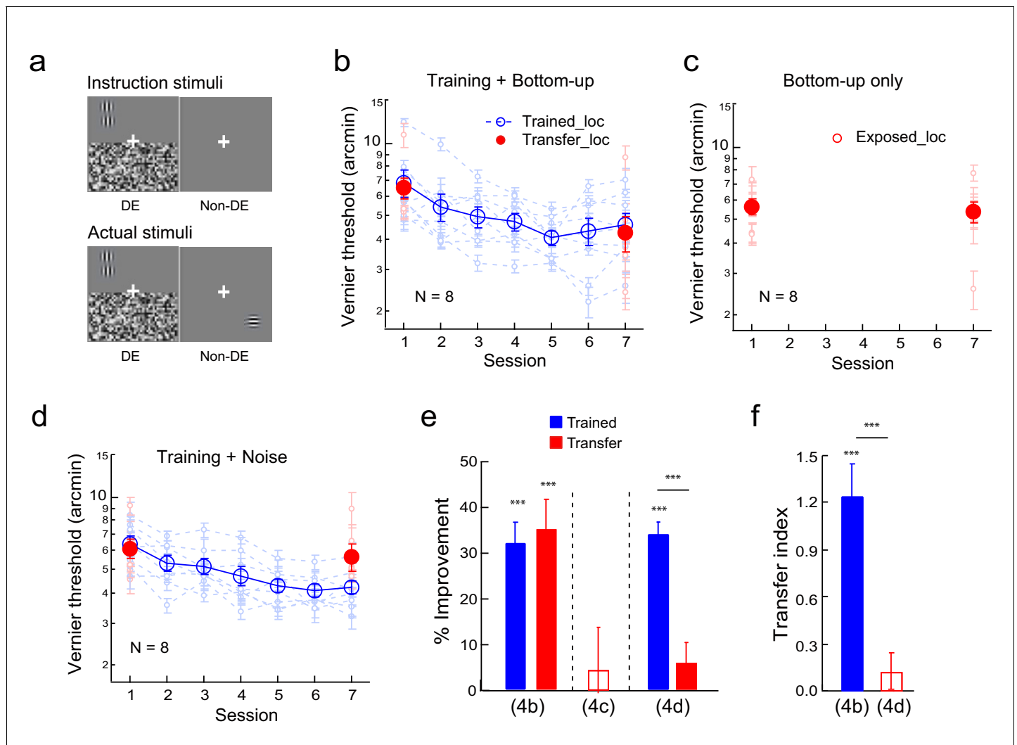
Figure 4. The effects of bottom-up stimulation of the transfer location on Vernier learning transfer. (a) CFS configurations for the simultaneous Vernier training and bottom-up stimulation of the diagonal transfer location. Instruction stimuli: The observer was instructed before the experiment to perform the Vernier task in the dominant eye, while flashing noise patterns covered the opposite visual hemifield across the horizontal meridian. A blank screen was shown to the non-dominant eye. Actual stimuli: A horizontal Gabor was simultaneously flashed in the non-dominant eye at the diagonal transfer location. The observers were neither told, nor were they aware of, the presence of the Gabor stimulus. (b) The mean and individual learning and transfer data with training and bottom-up stimulation of the transfer location. (c) Control experiment. Same as 4b except that there was no Vernier training. (d). Control experiment. Same as 4b except that there was no presence of the Gabor stimulus at the transfer location. (e). A summary of learning and transfer in the training plus bottom-up stimulation condition, the bottom-up stimulation alone condition, and the training plus noise-only condition. (f). A summary of the transfer indices in the training plus bottom-up stimulation condition and the training plus noise-only condition. Error bars indicate \pm 1 standard error of the mean. DE - dominant eye. * p < 0.05 ; ** p < 0.01 ; *** p < 0.001 . See Figure 4—source data 1 for raw data. DOI: 10.7554/eLife.14614.009
