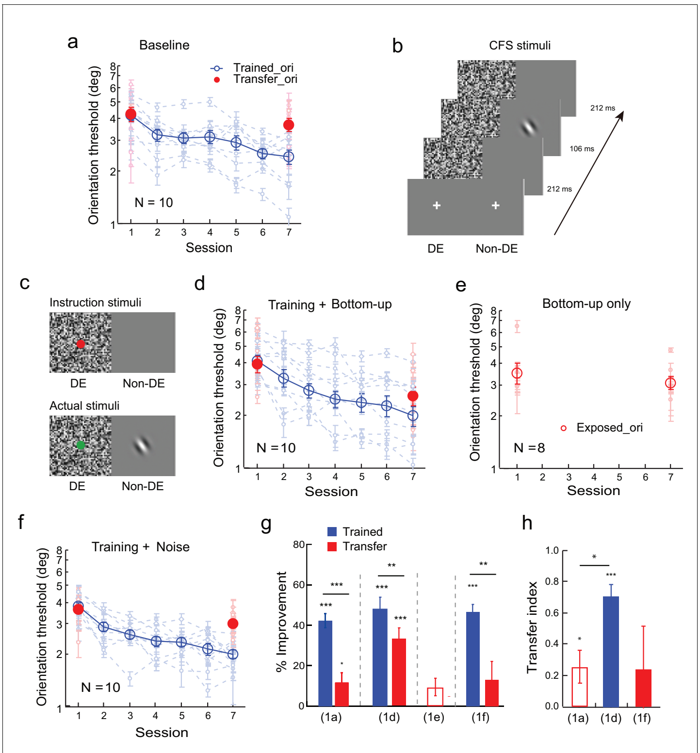
Figure 1. Orientation discrimination learning and the effect of bottom-up stimulation of the transfer orientation on learning transfer. (a) The baseline. Training was conducted at one orientation and the transfer of learning was tested at an orthogonal orientation to reveal orientation specificity. (b) CFS configurations for subconscious presentation of a Gabor at the orthogonal transfer orientation. The flashing noise was presented from 0 to 530 ms in the dominant eye. From 212 to 318 ms, a Gabor at the transfer orientation was also presented in the non-dominant eye. (c) Stimuli for bottom-up stimulation. Bottom-up stimulation was achieved by different CFS stimuli for instruction presentations before the experiment and for actual experimental presentations. Instruction stimuli: Before the experiment, the observers were instructed to report the color of a dot centered on the noise Figure 1 continued on next page
