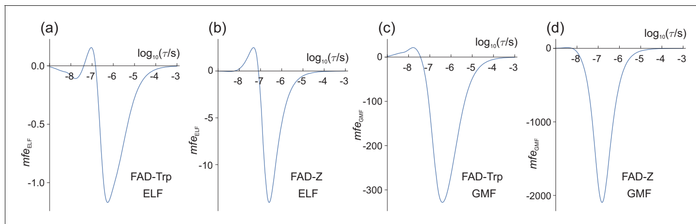
Figure 4. Magnetic field effects (in ppm) on model radical pairs as a function of the lifetime of the radical pair, \tau , in the range 1 ns–1 ms. The spin relaxation time is 1 \mu s. (a) and (c) A model of the [\text{FAD}^{\bullet-} \text{TrpH}^{\bullet+}] radical pair in cryptochrome, containing two ^{14}\text{N} nuclei in the \text{FAD}^{\bullet-} radical and one in the \text{TrpH}^{\bullet+} radical. (b) and (d) A model of the [\text{FAD}^{\bullet-} \text{Z}^{\bullet}] radical pair in cryptochrome in which the \text{Z}^{\bullet} radical has no hyperfine interactions. (a) and (b) mfe_{\text{ELF}} (Equation (10)) for B_0 = 50 \mu\text{T} , B_1 = 1.0 \mu\text{T} . (c) and (d) mfe_{\text{GMF}} (Equation (12)) for B_0 = 50 \mu\text{T} , \Delta B_0 = -1.0 \mu\text{T} . Note the different vertical scales of the four panels. The validity of the Taylor series expansion (Equation (9)) was confirmed by numerical integration over \alpha , the phase of the ELF field (Figure 4—figure supplement 1). Corresponding calculations for a spin relaxation time of 0.1 \mu s are shown in Figure 4—figure supplement 2. Corresponding versions of (a) and (c) when 25 \mu\text{T} \leq B_0 \leq 65 \mu\text{T} are shown in Figure 4—figure supplement 3.
