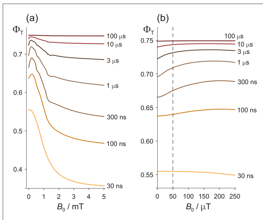
Figure 2. Effects of a static magnetic field on a model of the [\text{FAD}^{\bullet-} \text{TrpH}^{\bullet+}] radical pair in cryptochrome. (a) Dependence of the reaction yield \Phi_{\text{T}} on the static magnetic field strength, B_0 , for different values of the radical pair lifetime, \tau . The spin relaxation time is 1 \mu\text{s} . (b) An expanded view of the low field region of (a) with B_0 = 50 \mu\text{T} indicated by the dashed line. The difference between \Phi_{\text{T}} at zero field and at 50 \mu\text{T} is largest when \tau \approx 1 \mu\text{s} . The corresponding calculations for a spin relaxation time of 0.1 \mu\text{s} are shown in Figure 2—figure supplement 1 .
