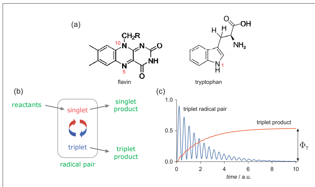
Figure 1. The radical pair mechanism. (a) Structures and atom numbers schemes for the FAD and TrpH molecules from which magnetically sensitive radical pairs are formed in purified cryptochromes. (b) Simple reaction scheme for a singlet-born radical pair able to react spin-selectively to form singlet and triplet reaction products. The red/blue arrows represent the coherent interconversion of the two forms of the radical pair. The reaction scheme is a simplified version of the cryptochrome photocycle ( Hore and Mouritsen, 2016; Maeda et al., 2012 ). (c) Schematic dependence of the amounts of triplet radical pair and triplet product present as a function of time (in arbitrary units) after the formation of the radical pair in a singlet state. The triplet yield, \Phi_T , is the amount of triplet product formed once all radical pairs have reacted.
