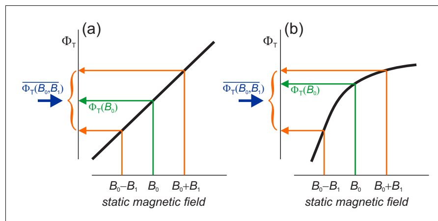
Figure 3. Schematic representations (thick black lines) of the dependence of the reaction yield, \Phi_{\text{T}} , on the strength of a static magnetic field. The orange arrows indicate the yields for the maximum and minimum values of B in Equation (5) . The green arrows show the yields when B = B_0 . The blue arrows mark the free radical yields averaged over the phase of the ELF field, Equation (6) . (a) When \Phi_{\text{T}} is linear in B , the effect of the GMF and the ELF field together equals that of the GMF alone. (b) When \Phi_{\text{T}} is non-linear, the effects of GMF plus ELF and GMF-alone differ. \Phi_{\text{T}} in (b) has been drawn with a negative curvature (concave downward), with the result that \overline{\Phi_{\text{T}}(B_0, B_1)} < \Phi_{\text{T}}(B_0) and mfe_{\text{ELF}} < 0 ( Equation (7) and (10) ). A positive curvature (concave upward) would give the opposite signs.
