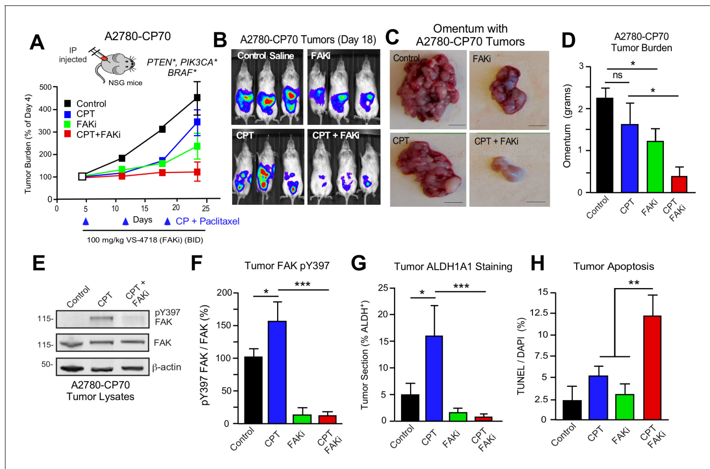
Figure 7. FAK inhibition sensitizes CP-resistant tumors chemotherapy-induced apoptosis. (A) Experimental schematic and IVIS imaging of labeled A2780-CP70 cells IP injected into NSG mice (randomized at Day 5). Experimental groups: control saline (black) injection on Days 5, 12, and 19; VS-4718 by oral gavage (green, 100 mg/kg, BID); CPT chemotherapy injection (blue, 3 mg/kg cisplatin and 2 mg/kg paclitaxel) on Days 5, 12, and 19; and VS-4718 plus CPT combined administration (red). IVIS imaging was performed on Days 4, 11, 18, and 23. Tumor burden is expressed as percent of Day 4. (B) Representative IVIS images of A2780-CP70 tumor burden on Day 18. (C) Representative images of omentum with A2780-CP70 tumors at Day 24. Scale is 0.5 cm. (D) Omentum-associated A2780-CP70 tumor mass ( n = 6 , \pm SEM * p < 0.05 , one-way ANOVA) from each treatment group. (E) A2780-CP70 tumor lysates immunoblotted for FAK pY397, FAK, and actin. (F) Ratio of pY397 FAK to total FAK levels in tumor lysates by immunoblotting. Values are means ( \pm SEM * p < 0.05 , *** p < 0.001 , one-way ANOVA) of three tumors per experimental group. Control set to 100. (G and H) Percent ALDH-1A1-positive immunofluorescent A2780-CP70 tumor staining or apoptosis (TUNEL and Hoescht 33342 staining) in A2780-CP70 tumors. Values are means ( \pm SEM, two independent tumors, five random fields per tumor at 20X, * p < 0.05 , ** p < 0.01 , *** p < 0.001 one-way ANOVA).
