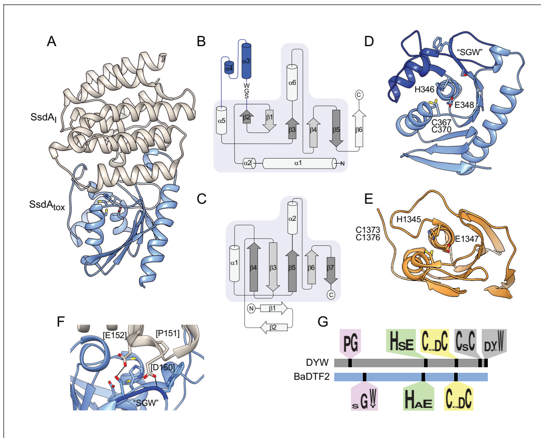
Figure 6. The structure of BaDTF2 member single-strand DNA deaminase toxin A (SsdA) bears little resemblance to double-stranded DNA deaminase A (DddA) and reveals motifs differentiating toxins from RNA-targeting DYW proteins. (A) Ribbon diagram depiction of the SsdA tox -SsdA I structure. (B,C) Secondary structure diagrams for SsdA tox and the core fold of deaminase superfamily proteins (Iyer et al., 2011). The SWG motif conserved in BaDTF2 toxins and the accompanying \alpha -helical insertion (blue) are indicated in B. (D) Active site view of SsdA tox . Catalytic and zinc-coordinating residues, SGW motif and \alpha -helical insertion (blue) are indicated. (E) Active site view of DddA tox indicating catalytic and zinc-coordinating residues. (F) Zoom-in view of the contact site between SsdA I and the active site of SsdA tox . (G) Conserved motifs identified in DYW and BaDTF2 proteins.
