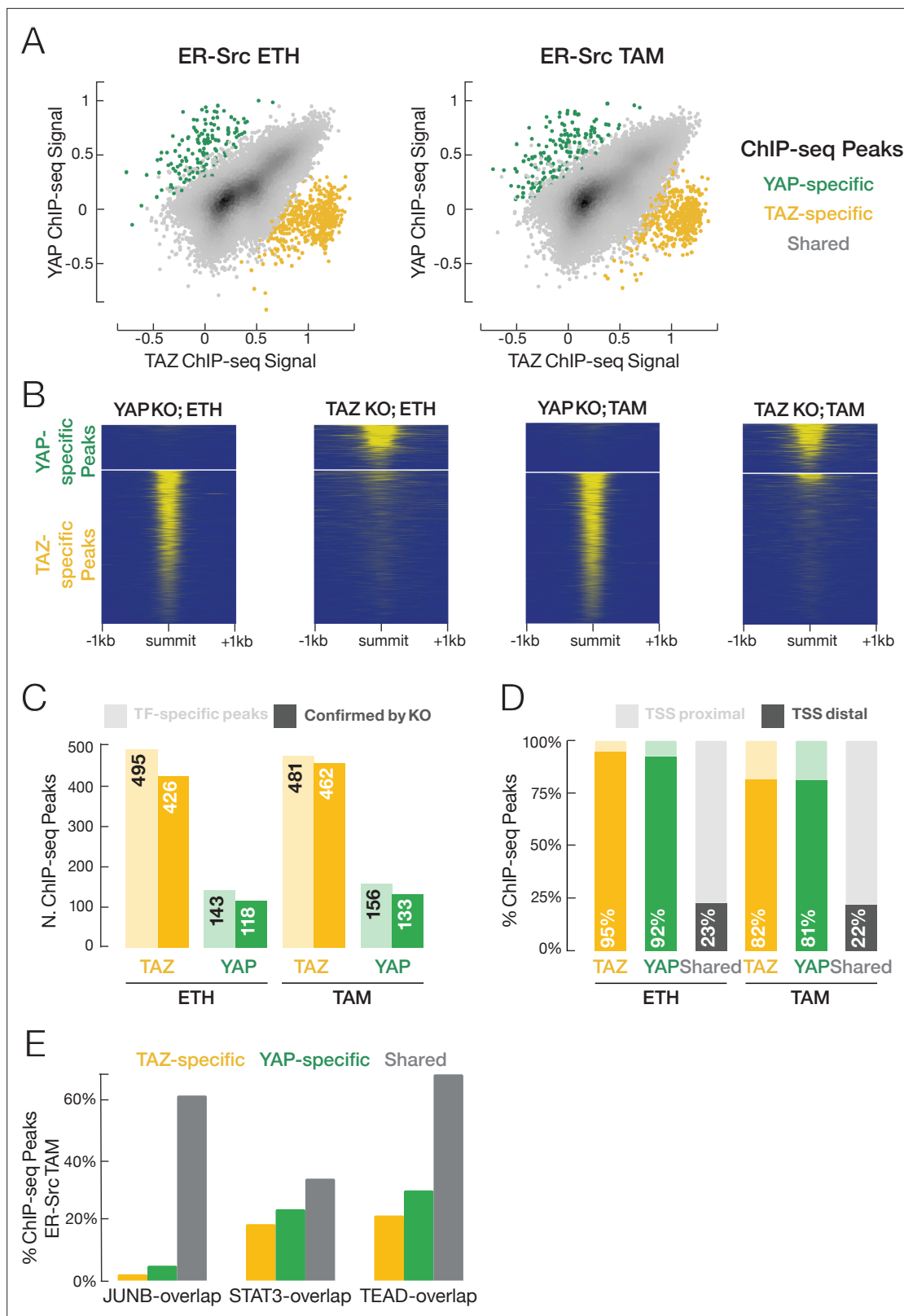
Figure 4. YAP and TAZ have highly similar binding profiles, but a small subset of binding sites is unique to each factor. (A) Correlation ( r \sim 0.7 ) of YAP and TAZ binding signals in non-transformed (ETH) and transformed (TAM) cells. Putative YAP- and TAZ-specific sites are indicated, respectively, as green and yellow. (B) YAP and TAZ binding signals in YAP- or TAZ-knockout cell lines using an antibody that recognizes both proteins. (C) Number of putative YAP- and TAZ-specific sites (lighter colors) confirmed in cells deleted for the indicated factor (darker colors). (D) Percentage of YAP-specific, TAZ-specific, Figure 4 continued on next page
