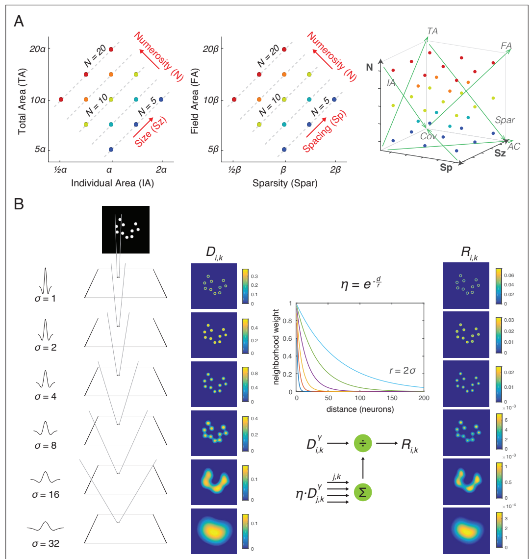
Figure 1. Stimulus design and computational methods. (A) Properties of magnitude dimensions represented in three orthogonal axes defined by log-scaled number (N), size (Sz), and spacing (Sp) (Table 1). (B) Schematic illustration of the computational process from a dot-array image to the driving input (i.e., the model without divisive normalization), D , of the simulated neurons, versus the normalized response (i.e., the model with divisive normalization), R . A bitmap image of a dot array was fed into a convolutional layer with DoG filters in six different sizes (Equation 1). The resulting values, after half wave rectification, represented the driving input. Neighborhood weight, defined by \eta , was multiplied by the driving input across all the neurons across all the filter sizes, the summation of which served as the normalization factor (see Equations 2 and 3). This illustration of \eta is showing the case where r is defined by twice the size of the sigma for the DoG kernel. DOG, difference-of-Gaussians.
