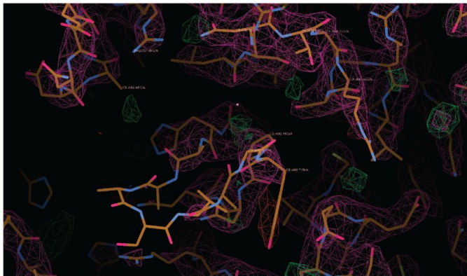
TcoPYK -sdAb42 (PDB ID: 8RTL)
