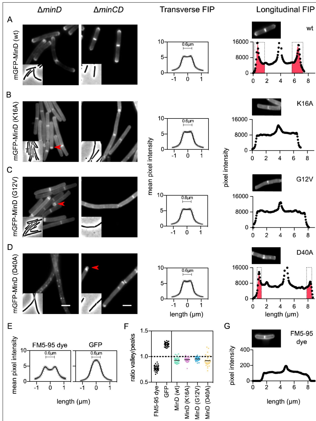
Fig. 1. Localization of monomeric and dimeric MinD variants
