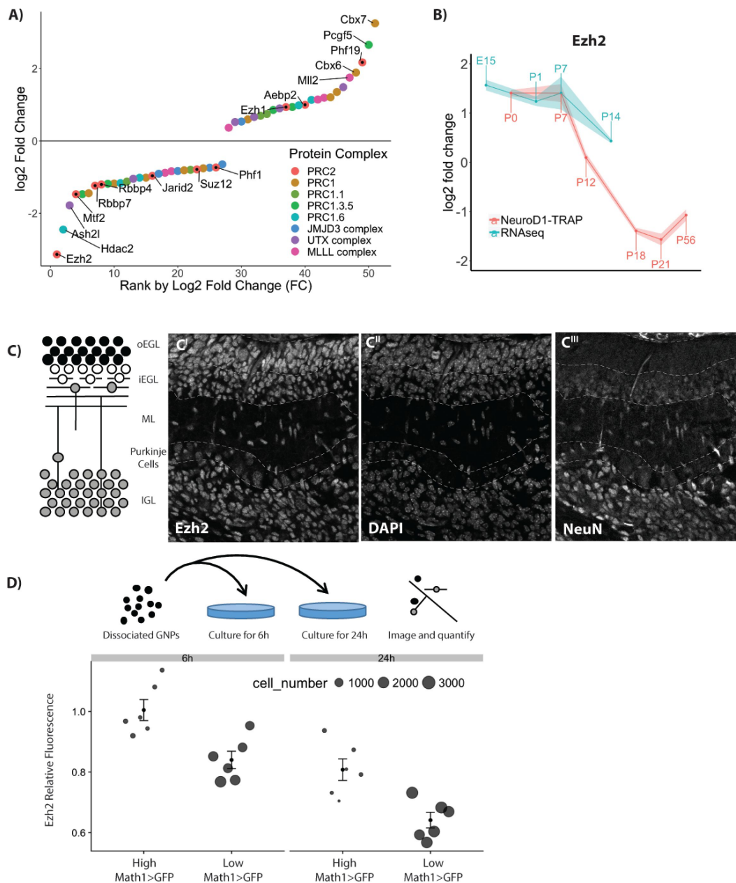
Figure 5 Transcriptional regulation of known H3K27me3 effector protein complexes during granule neuron (GN) development.
