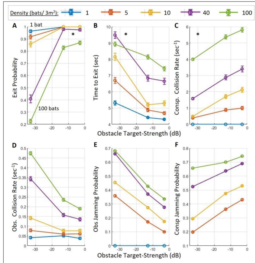
Supplementary Figure 3. Sensitivity of exit performance to obstacle target strength.
