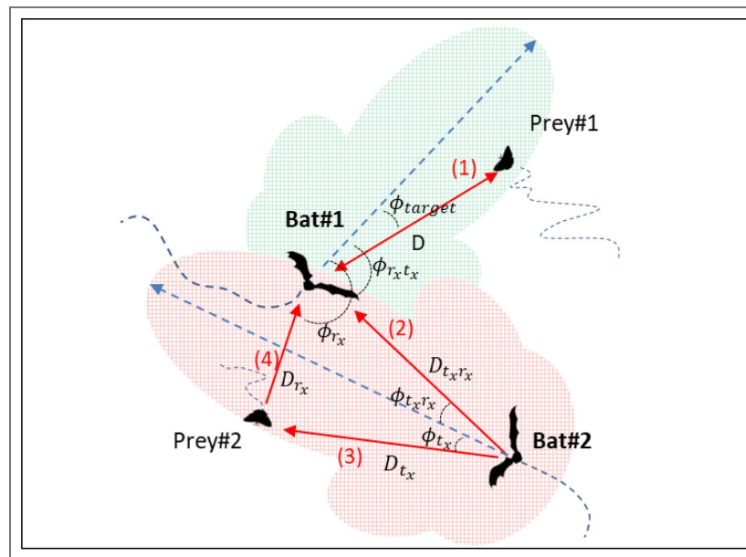
Supplementary Figure 5. Angles and distances for two bats and two reflecting objects.
