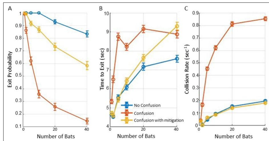
Figure 4. The impact of confusion on performance.
