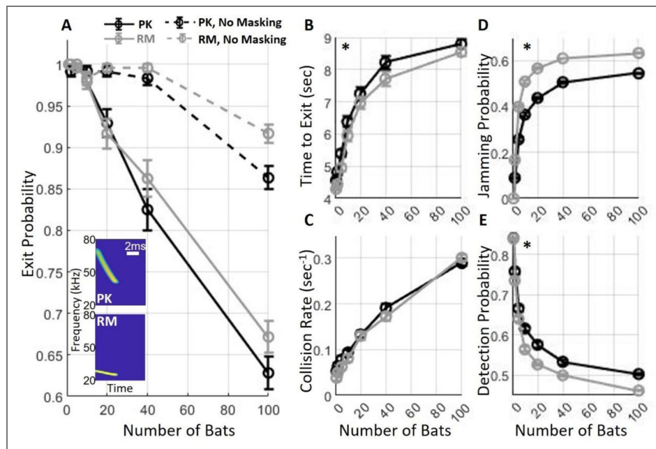
Figure 2. Exit performance of P. kuhlii (PK) and R. microphyllus (RM).
