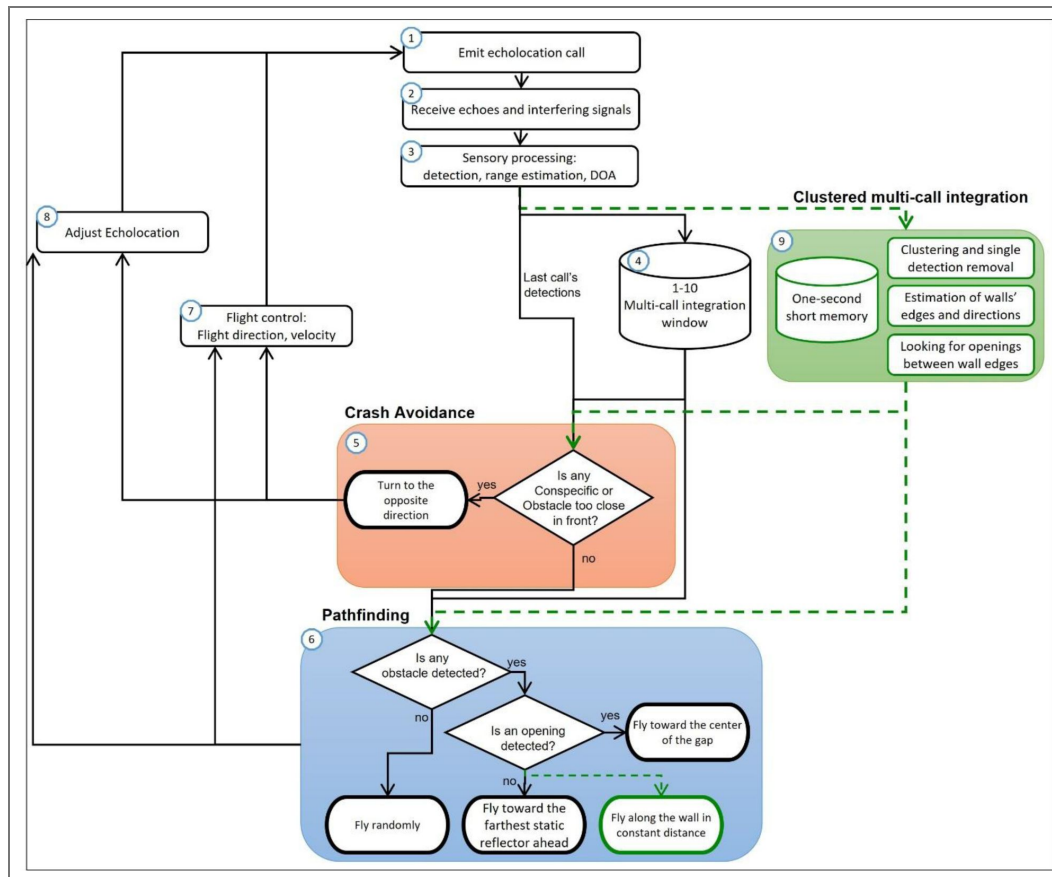
Supplementary Figure 1. Decision-making in echolocation-based pathfinding.
