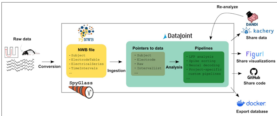
Figure 1. Overview of Spyglass.
