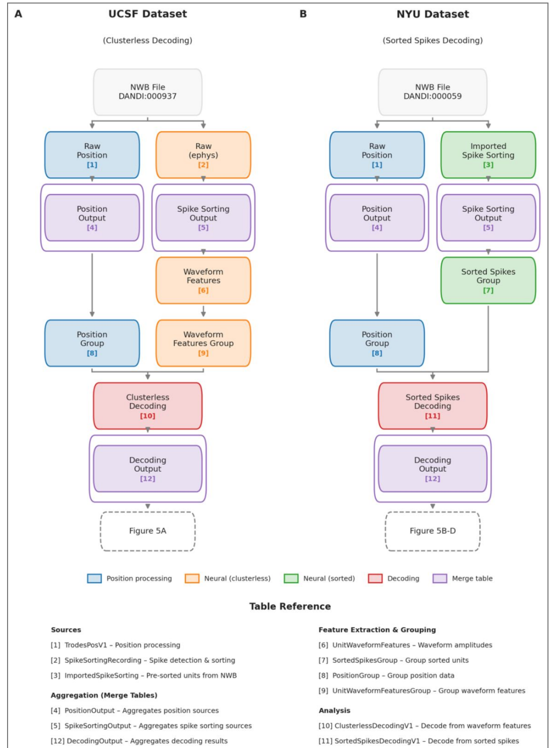
Supplemental Figure 1. Spyglass pipeline workflow for Figure 5A and B. (A) Decoding of the UCSF dataset started with the NWB file. Data was ingested into the RawPosition and Raw tables, which hold the unprocessed position data (only LED tracking from the Trodes hardware system) and the electrophysiology traces respectively. Position data from the two LEDs had outliers removed, interpolated over, and then smoothed and combined into a single head position via the TrodesPosV1 table (and requisite Selection and Parameter tables which specified the dataset and the parameters for processing). This was then inserted into the PositionOutput merge table. The position data was then inserted into the PositionGroup table which in this case is a passthrough table (but in
