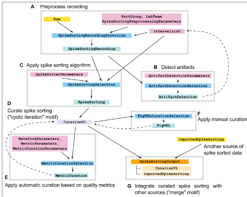
Figure 3. Spike sorting pipeline.
