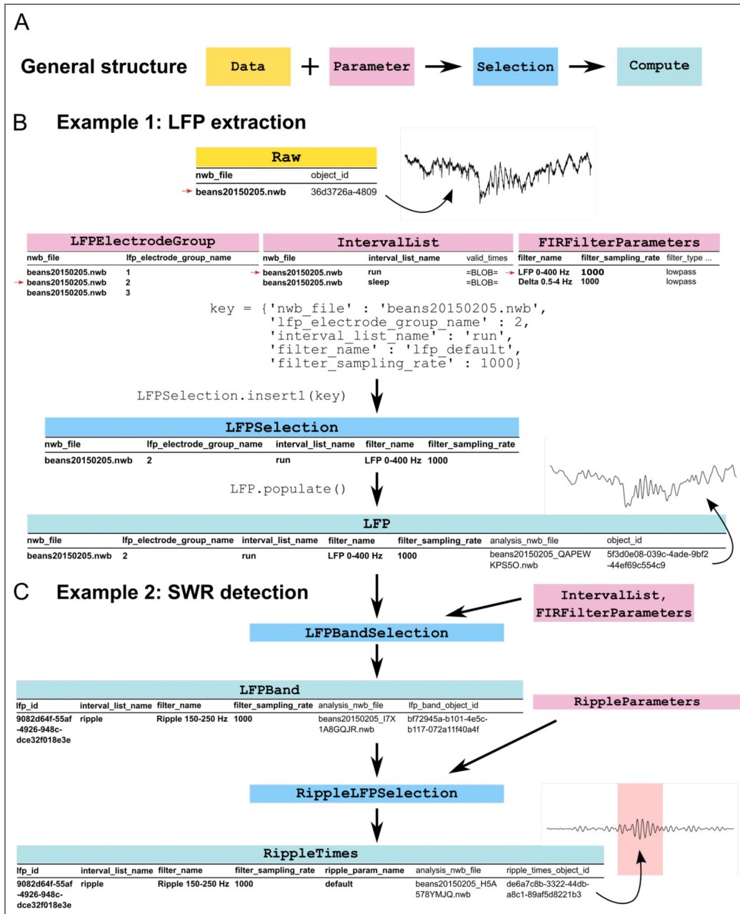
Figure 2. Analysis pipelines in Spyglass.
