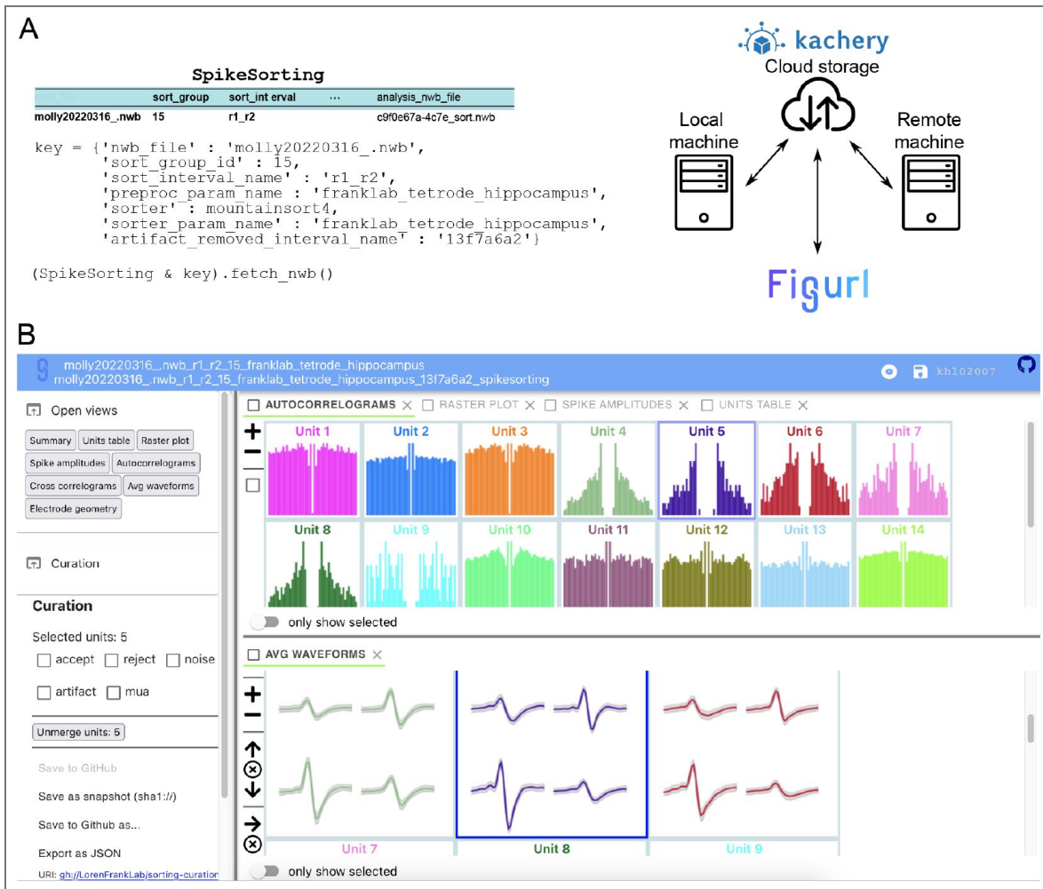
Figure 4. Sharing data and visualizations.
