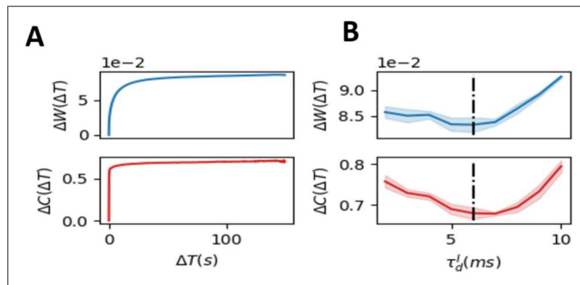
Figure 7. Structural mechanism underlying restricted representation.
