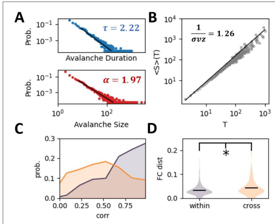
Figure 1. Variable spontaneous dynamics in the experimental data.
