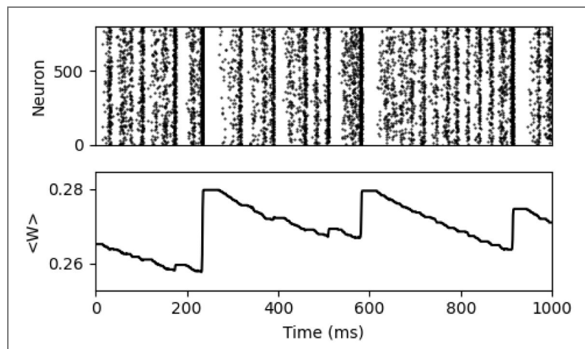
Figure S4. Raster plot of the plasticity model at the supercritical state with \tau_d^I = 10ms and the corresponding dynamics of the average synapse strength.
