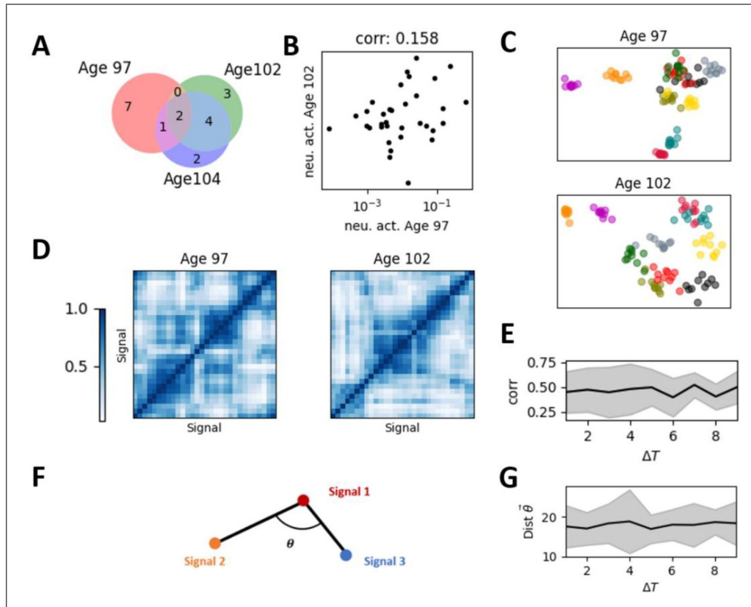
Figure 2. Representational drift and the restricted representational geometry in the experimental data.
