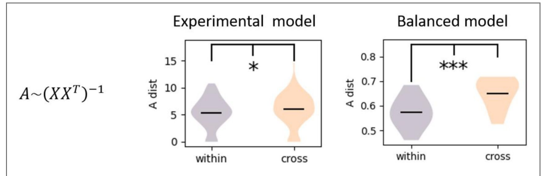
Figure S1. The estimated effective connectivity from neural activity using inverse of co-variance matrix. Both experimental data (two sample t test, p \approx 0.03 < 0.2 ) and balanced model (two sample t test, p \approx 0 ) show larger change in effective connectivity for the cross-session than the within-session.
