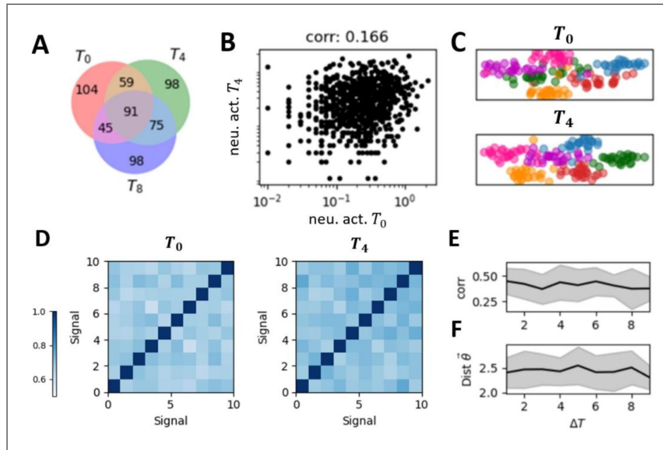
Figure 4. Representational drift and the restricted representational geometry in the self-organized critical (SOC) model.
