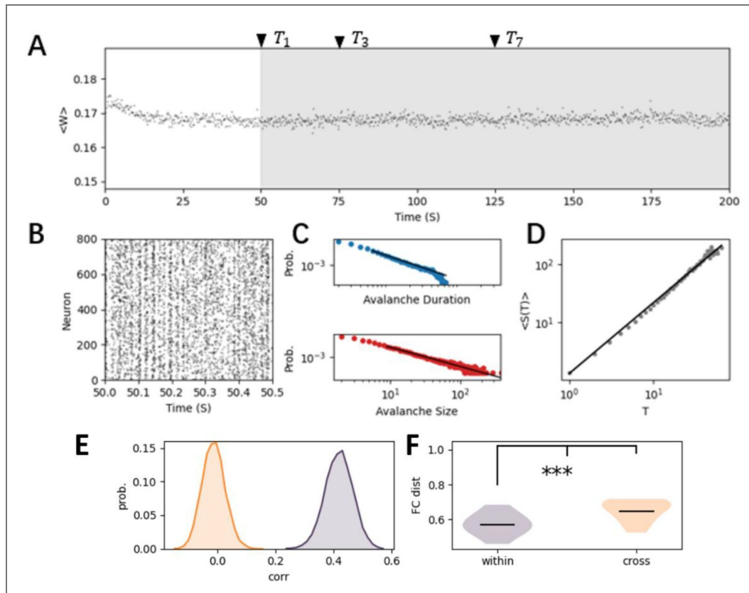
Figure 3. The self-organized criticality (SOC) in the E-I network with homeostatic plasticity.
