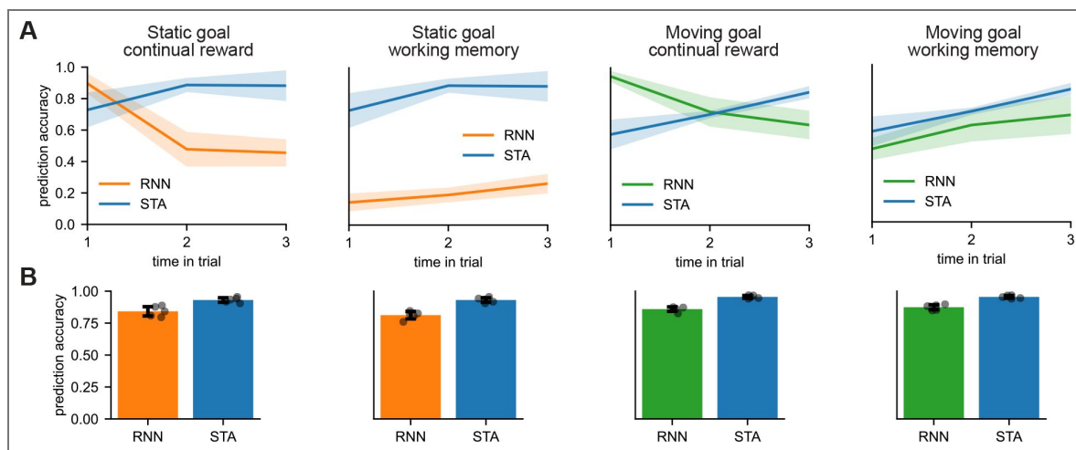
Figure S3. RNNs trained on simpler tasks do not learn spacetime representations.
