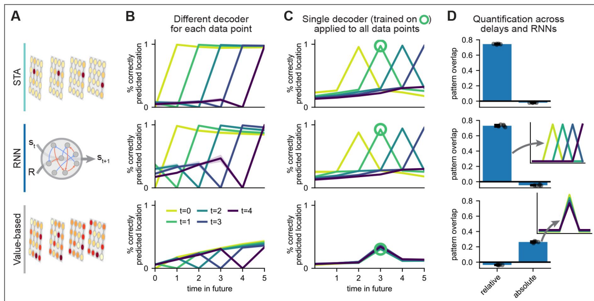
Figure S2. Additional analyses of learned RNN representations.
