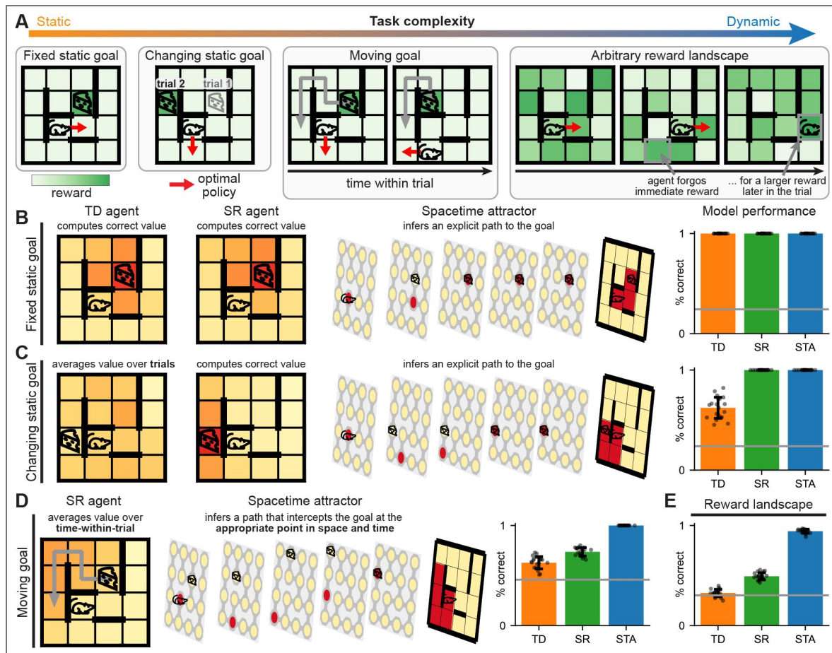
Figure 3. Model comparisons in static and dynamic tasks.
