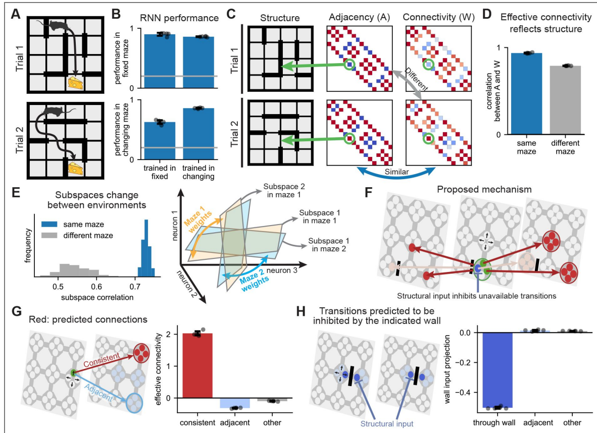
Figure 6. Spacetime attractors can adapt to changing structure.
