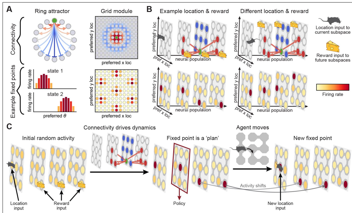
Figure 2. The spacetime attractor.
