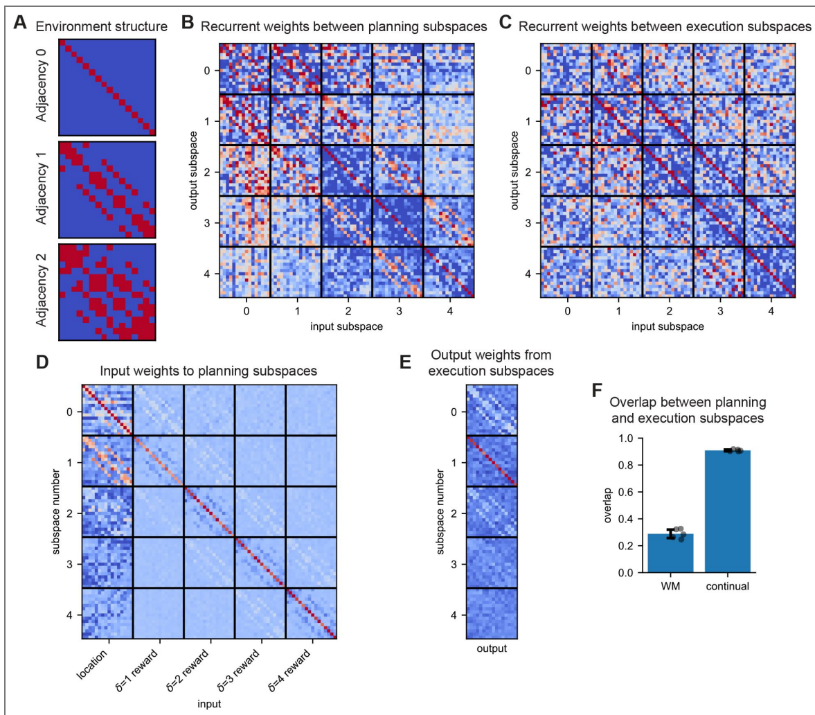
Figure S4. Parameters learned by the reward landscape RNN.
