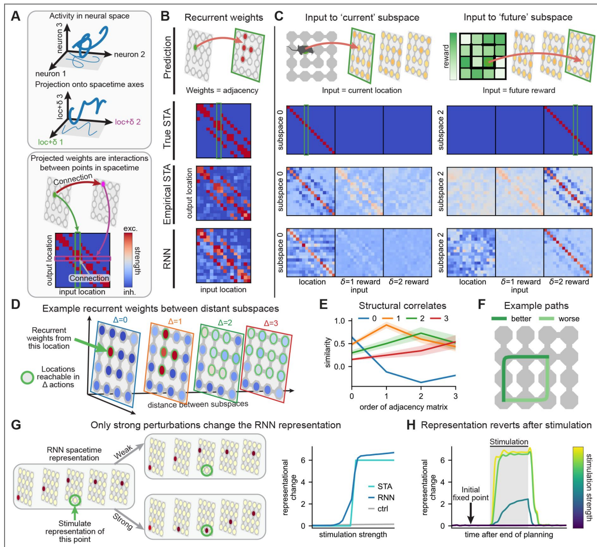
Figure 5. RNNs learn a world model.
