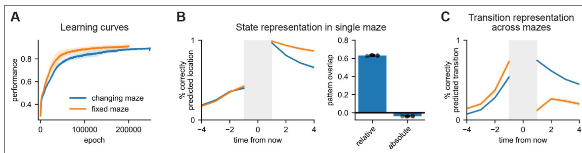
Figure S9. Additional analyses of RNNs trained with changing environment structure.
